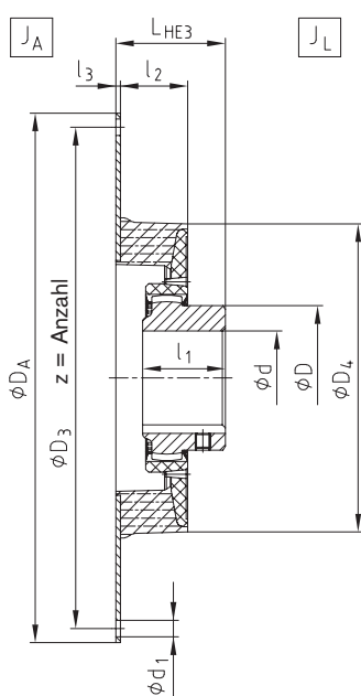
Bauart HE3
