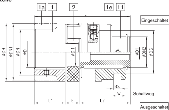
Bauart SD
