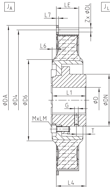
Bauart AK
