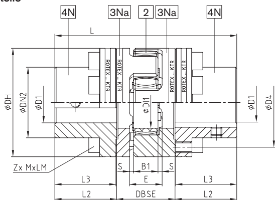
Bauart AFN
