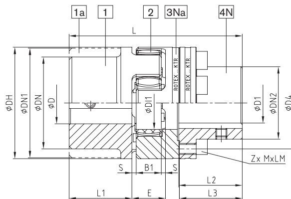
Bauart BFN
