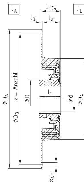
Bauart HE4
