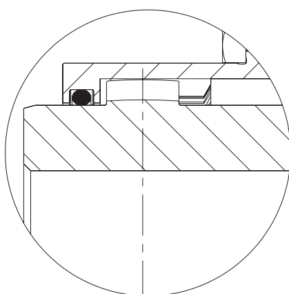
Bauart FR
